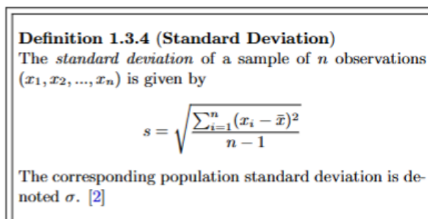
Figure 3: Standard Deviation
