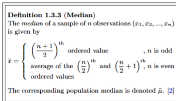
Figure 2: Median
